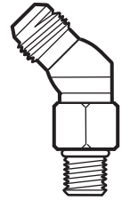
160-053 9/16-18 to #8 JIC 45°
