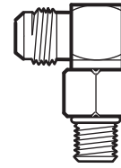
160-054 9/16-18 to #8 JIC 90°
